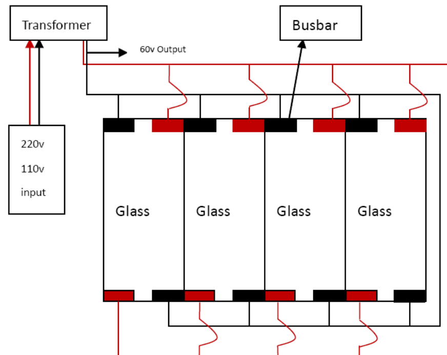
Double side wiring
