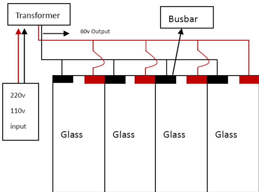
Single side busbar wiring
